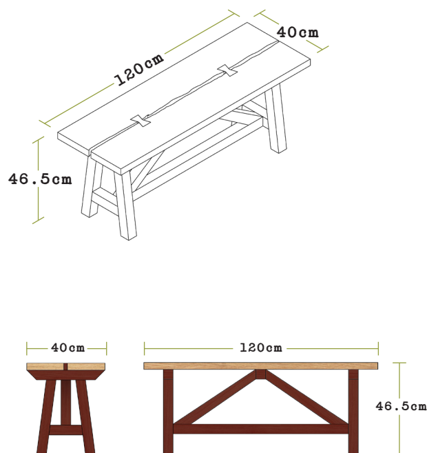
Bench Elevations
