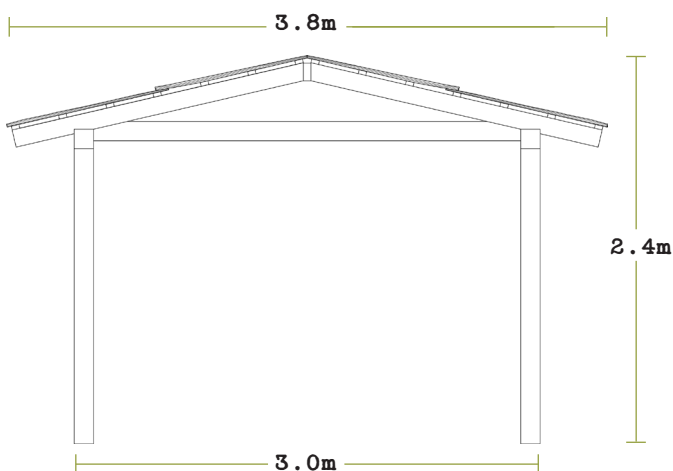
Pavilion Elevations
